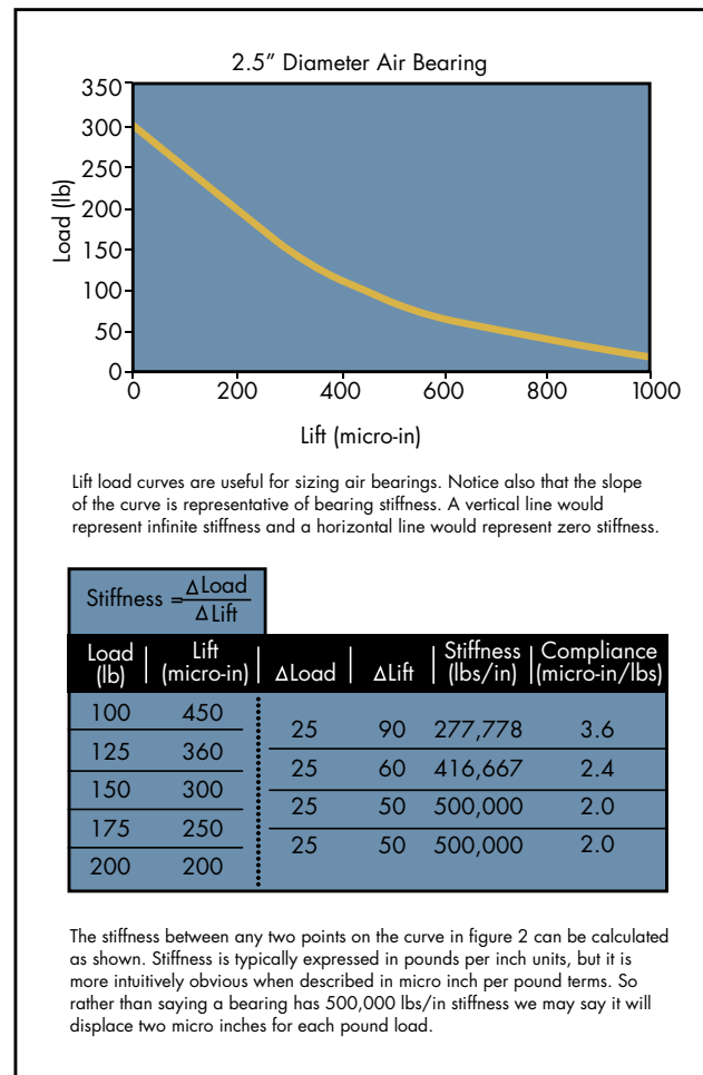
Figure 4 - Air Bearing Stiffness
