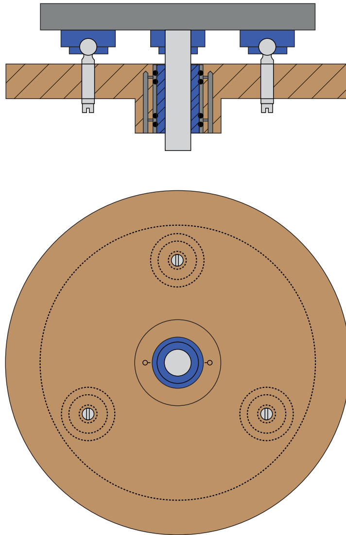
Figure 25 - Rotary Table
