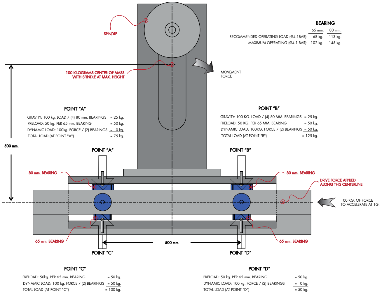
Figure 15 - Dynamic Loading
